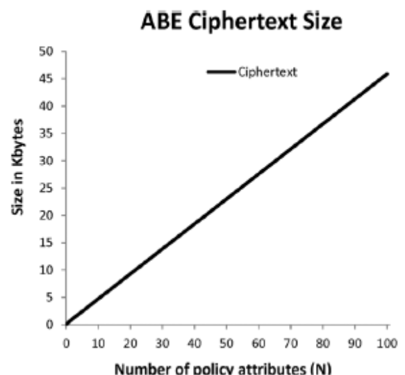
Figure 2.3.1(a) Calculating cipher text size
