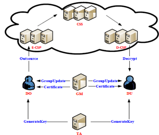
Figure 2.1 Architecture of Storage System
