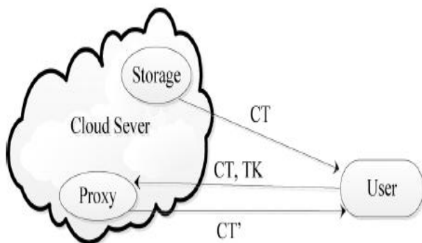
Figure 2.3.2 Cipher Text Policy-Attribute Based Encryption System with outsourced decryption Intermediary re encryption: In Cipher Text Policy-Attribute Based Encryption with redistributed unscrambling, a customer outfits the cloud with a change key that allows the cloud to unravel a Cipher Text Policy-Attribute Based Encryption figure message on message into an essential figure message on the comparable, without grabbing anything about. This is reminiscent of the possibility of middle person re encryption. Delegate re encryption allows a middle person, using are encryption key, to change an encryption of under Alice's open key into an encryption of the identical under Bob's open key without the mediator grabbing anything about the encoded
